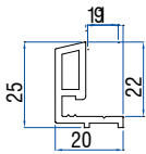
Mesh Adaptor 50502 - 11041
